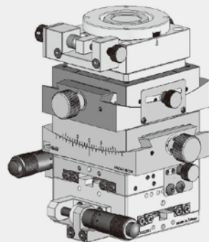
Micro-alignment module for AOI system.
