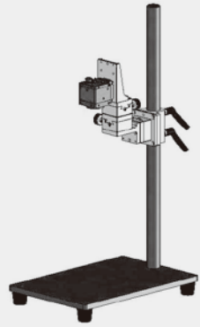
Simplified & rapid adjustment module for CCD monitoring.
